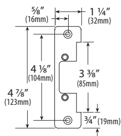
CX-ESF-2: Aluminum Finish CX-ESF-2BZ: Dark Bronze Finish ANSI Round
